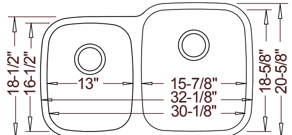
Product Diagram
